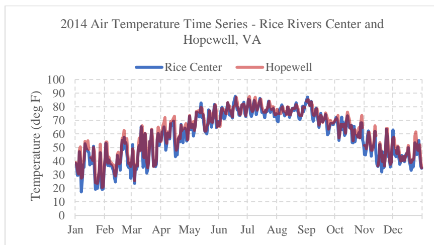
Figure 4.1.2. 2014 daily air temperature time series data (°F) for the VCU Rice Rivers Center and Hopewell, VA.
