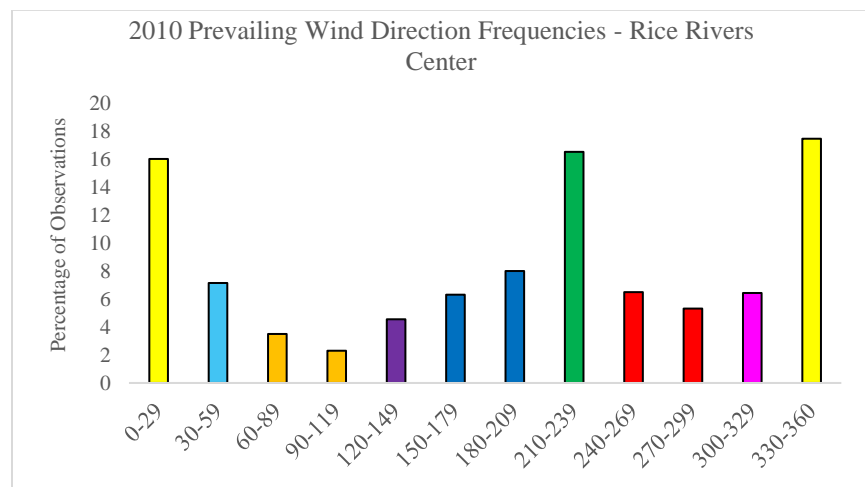
Figure 4.3. 2010 prevailing wind direction frequencies (%) for the Rice Rivers Center
